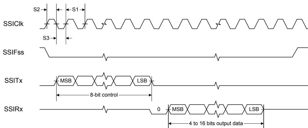
Figure 27-14. SSI Timing for MICROWIRE Frame Format (FRF=10), Single Transfer
